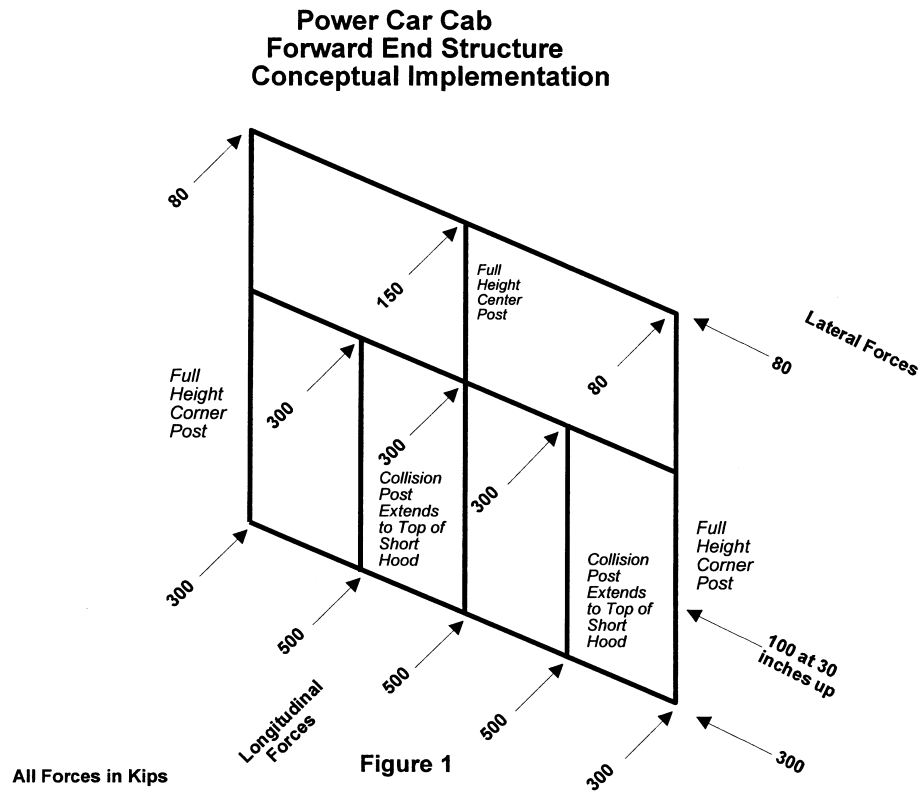
FIGURE 1 TO SUBPART E OF PART 238—POWER CAR CAB FORWARD END STRUCTURE CONCEPTUAL IMPLEMENTATION
