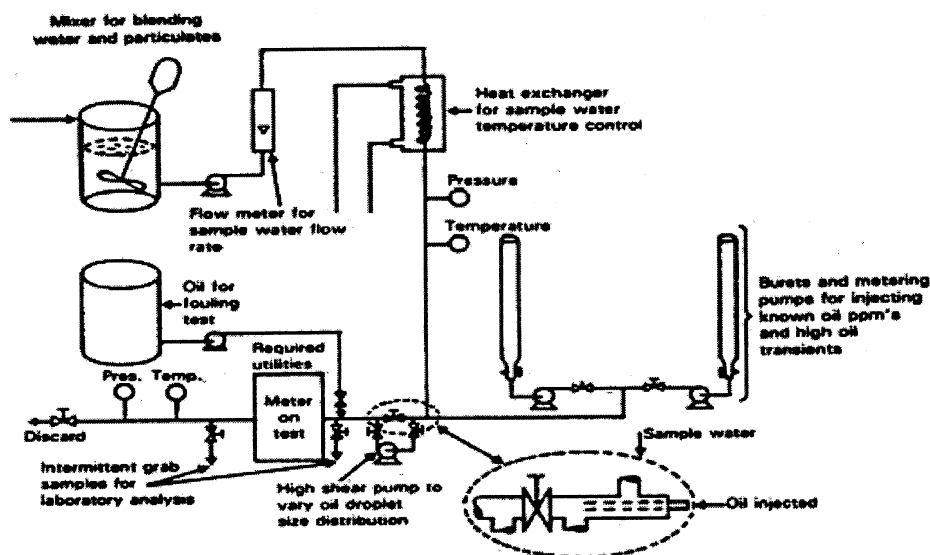
FIGURE 162.050-19—MONITOR AND BILGE ALARM TEST RIG
