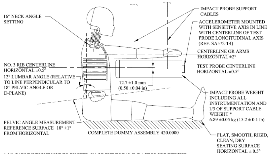
FIGURE T5 TORSO FLEXION TEST SETUP SPECIFICATIONS
