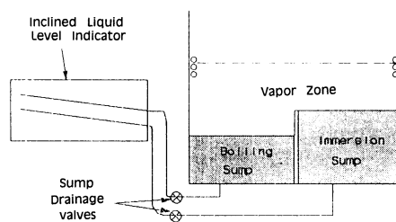
Figure 307-2. Solvent Cleaner Test Setup.
