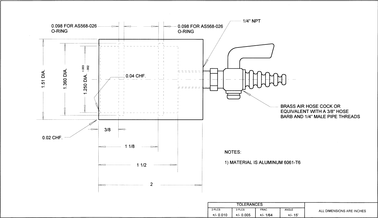
FIGURE L-30. FLOW RATE MEASUREMENT ADAPTER
