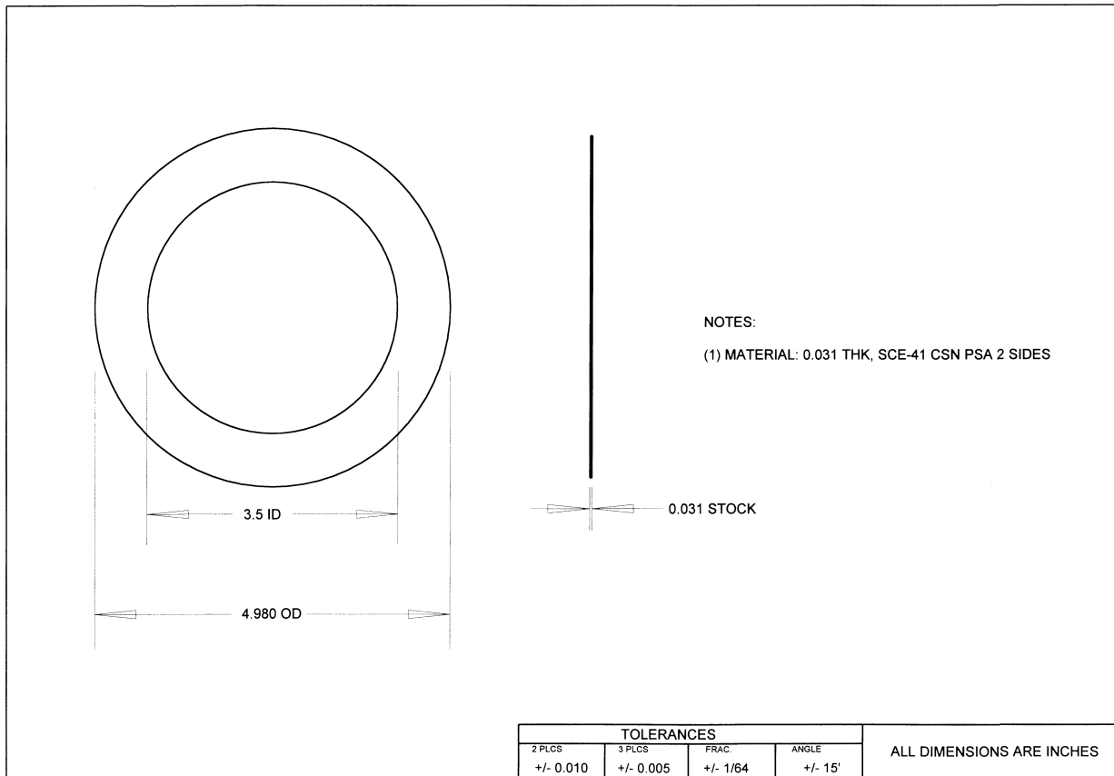
FIGURE L-6. 10-MICRON GASKET
