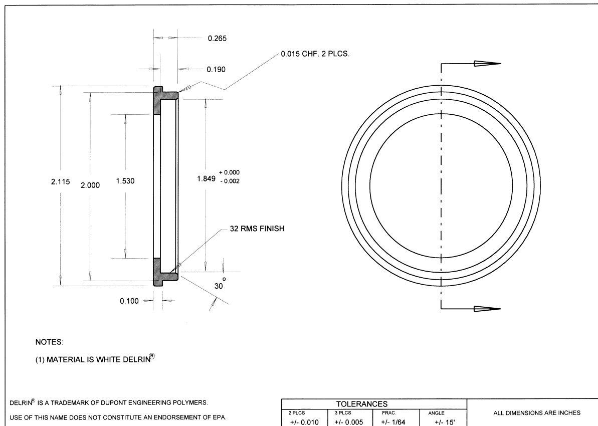
FIGURE L-29. FILTER CASSETTE, LOWER SECTION
