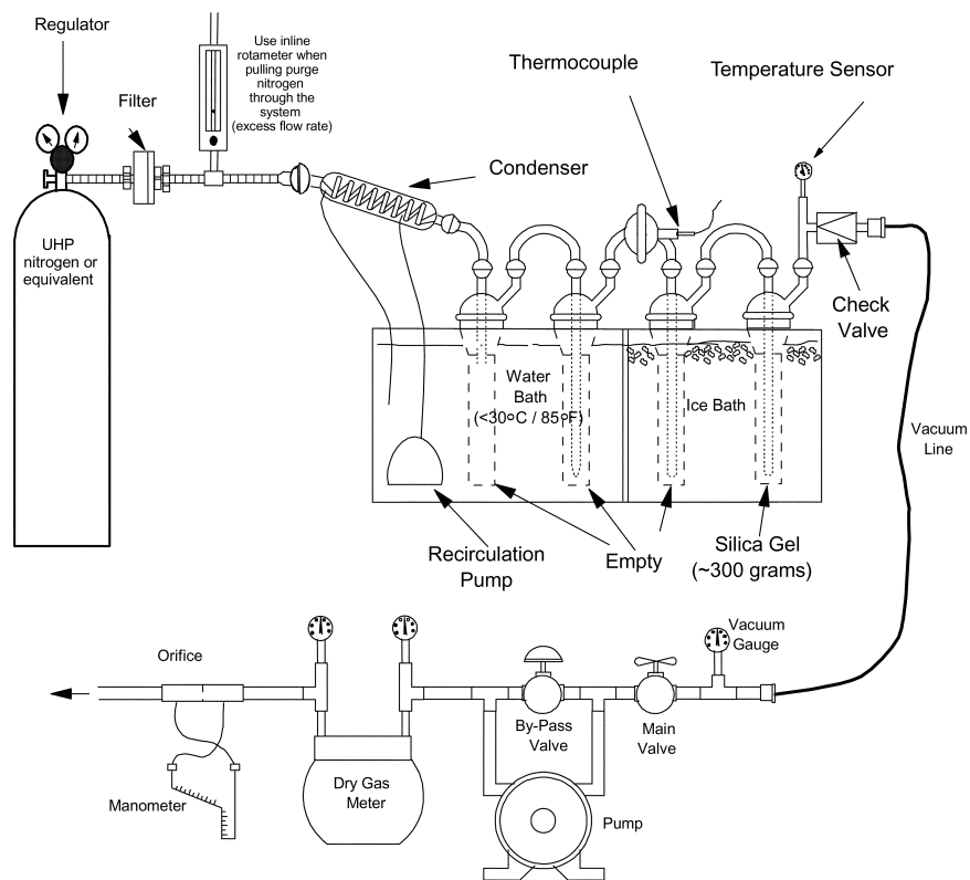
Figure 2. Nitrogen Purge Train Configuration (Vacuum Purge)
