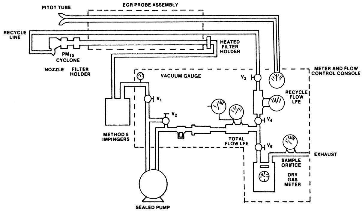
Figure 1. Schematic of the exhaust gas recycle train.
