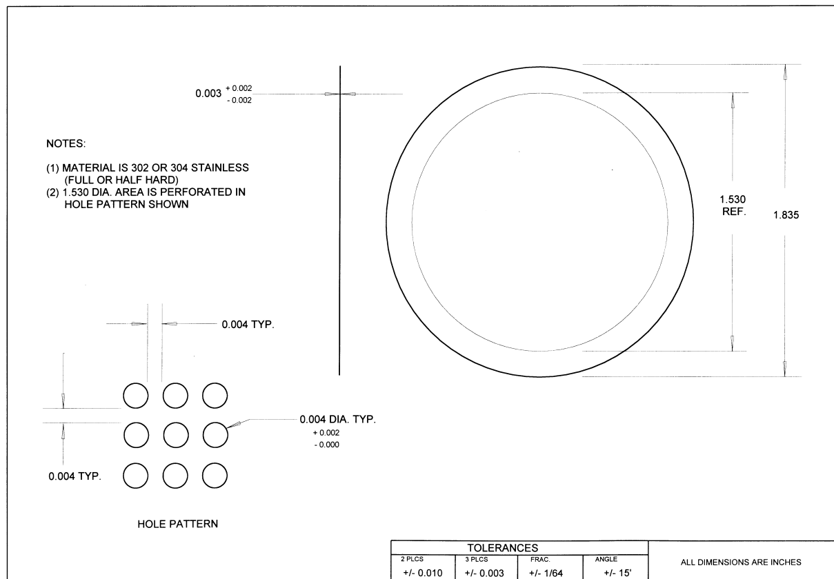
FIGURE L-28. FILTER SCREEN
