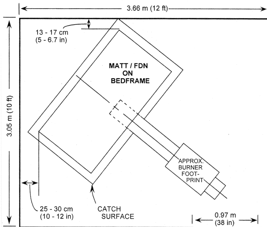
FIGURE 2 TO PART 1633—TEST ARRANGEMENT IN 3.05M X 3.66M (10 FT X 12 FT) ROOM (CONFIGURATION B)
