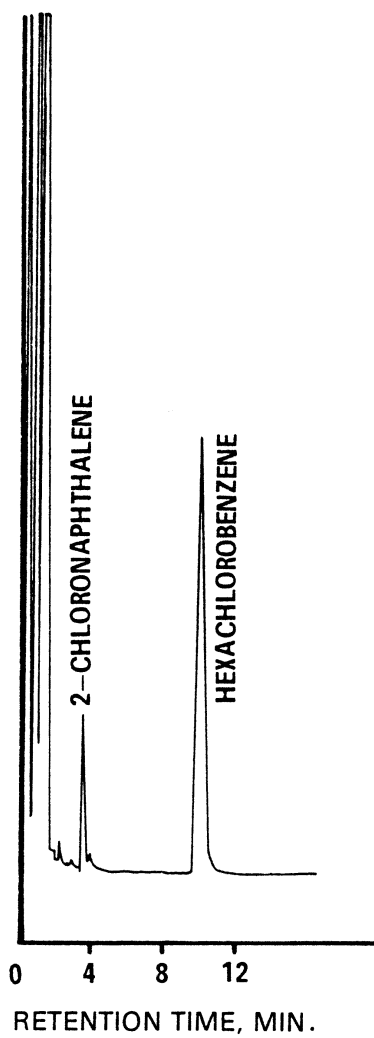
Figure 2. Gas chromatogram of chlorinated hydrocarbons.
