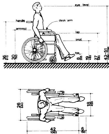
Fig. A3 Dimensions of Adult-Sized Wheelchairs
