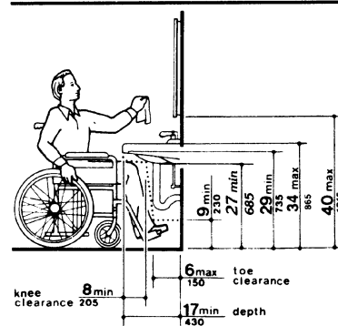
Fig. 31 Lavatory Clearances
