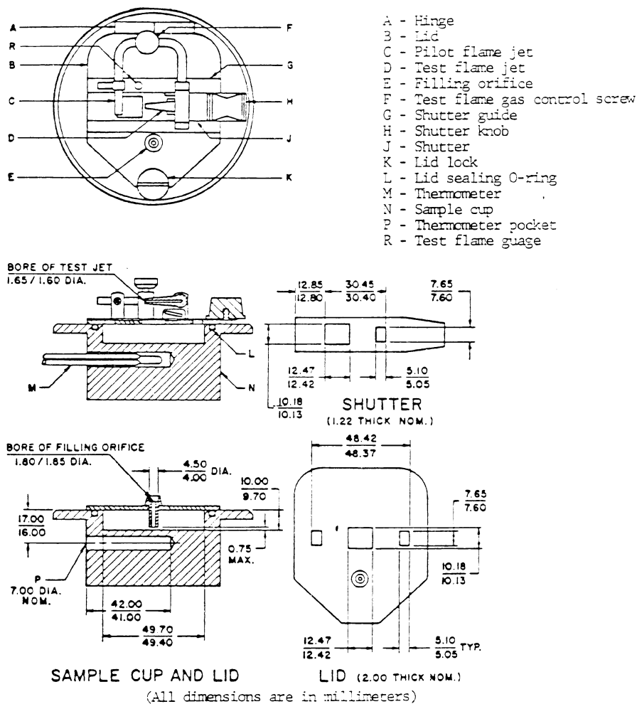
FIGURE 1 - Closed-cup tester
