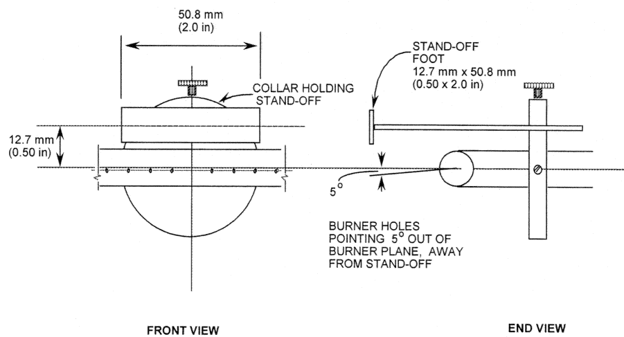
FIGURE 5 TO PART 1633—DETAILS OF BURNER STAND-OFF
