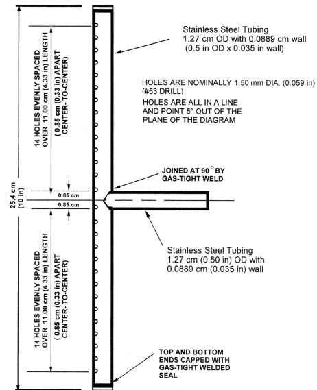
FIGURE 4 TO PART 1633—DETAILS OF VERTICAL BURNER HEAD
