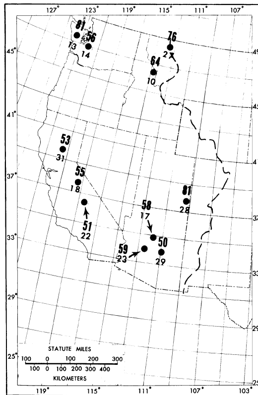
Plate 5: Observed rainfalls \geq 50\% of all-season PMP, U.S. west of the Continental Divide for 1000 \text{ mi}^2 for one duration between 6 and 72 hours. (Large number is % of PMP. Small number is storm index, see table 2.)
