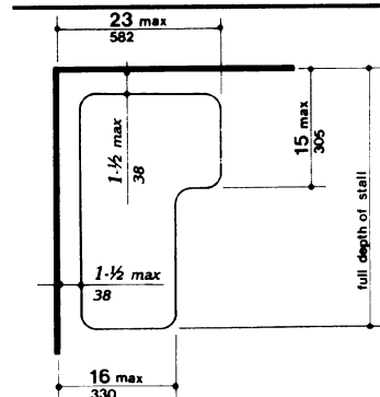
Fig. 36 Shower Seat Design
