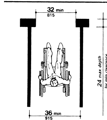
Fig. 1 Minimum Clear Width for Single Wheelchair
