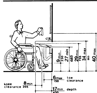
Fig. 31 Lavatory Clearances
