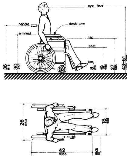
Fig. A3 Dimensions of Adult-Sized Wheelchairs
