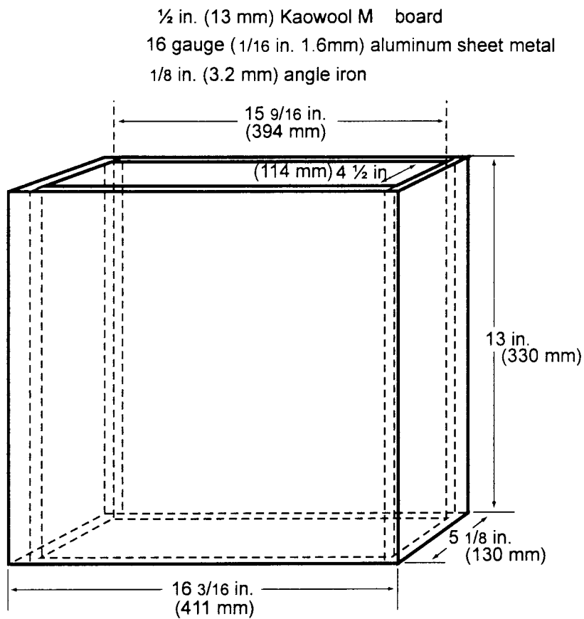
Figure 2 - Internal Chimney
