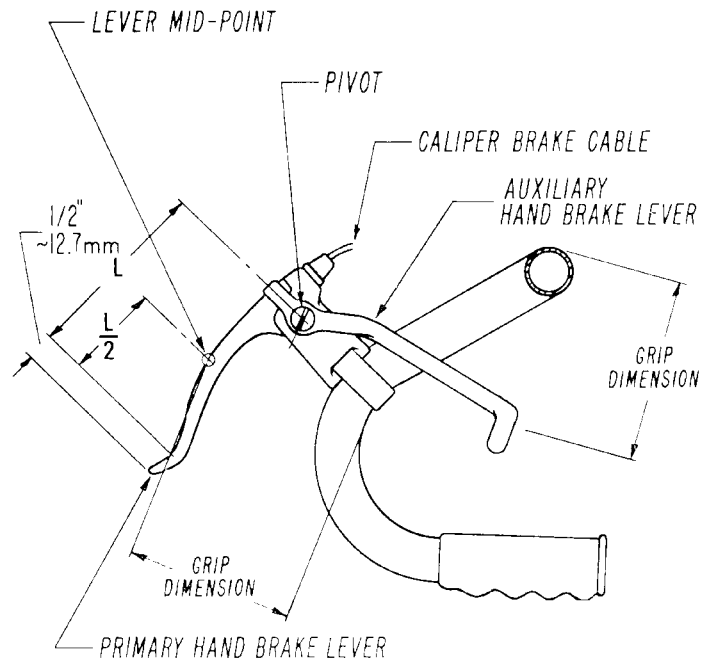
FIG. 5-TYPICAL HANDBRAKE ACTUATOR SHOWING GRIP DIMENSION
