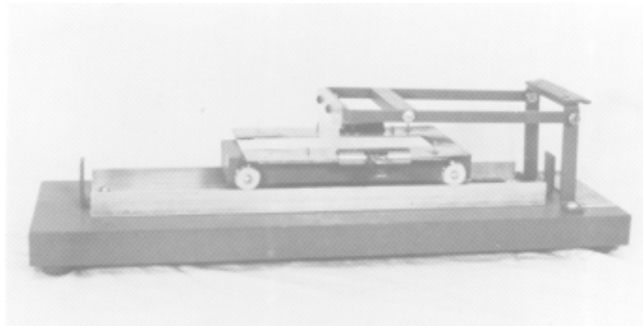
FIGURE 3—BRUSHING DEVICE. 1
