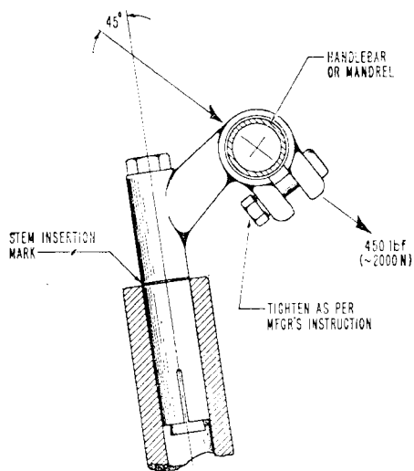
FIG 2—HANDLEBAR STEM LOADING
