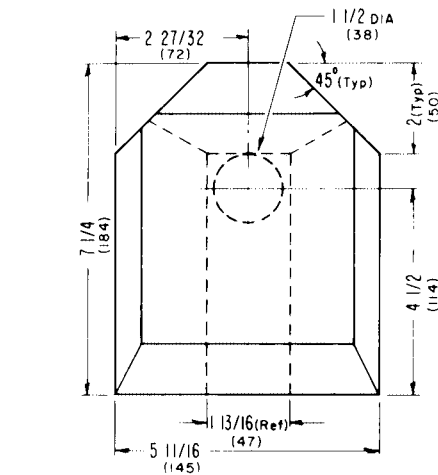
FIG 2-HEADFORM PROBE
