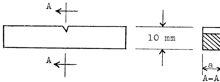
CHARPY V-NOTCH SPECIMEN
