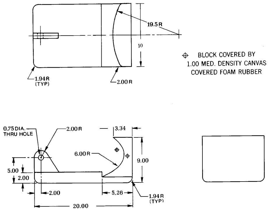
FIGURE 2 – BODY BLOCK FOR LAP BELT
