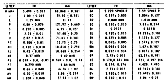
Fig. 18 - Dimensional Specifications for Integral Mount Sealed Beam Headlamps, Types G and H
