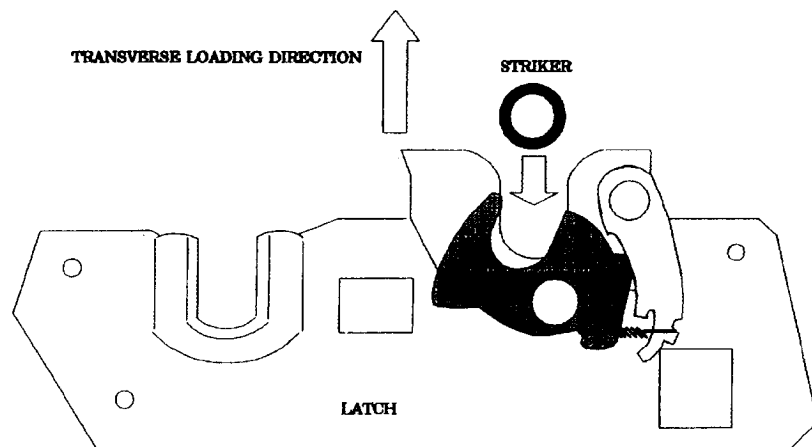
Figure 1.- Top View of a Typical Back Door Latch
