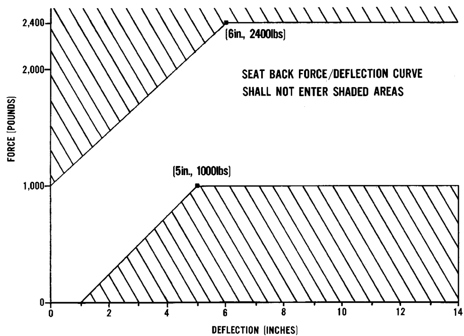
FIGURE 1 - FORCE/DEFLECTION ZONE
