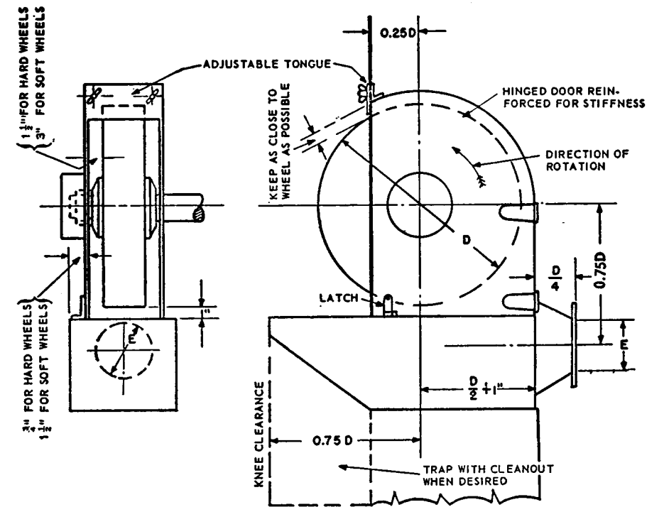
STANDARD BUFFING AND POLISHING HOOD
