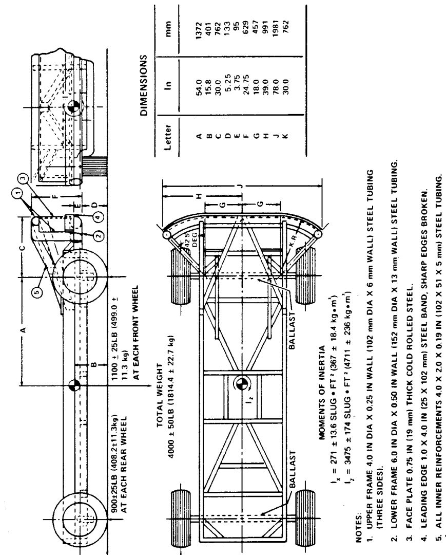
FIG. 2—COMMON CARRIAGE WITH CONTOURED IMPACT SURFACE ATTACHED
