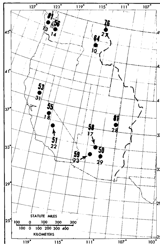
Plate 5: Observed rainfalls > 50\% of all-season PMP, U.S. west of the Continental Divide for 1000 \text{ mi}^2 for one duration between 6 and 72 hours. (Large number is % of PMP. Small number is storm index, see table 2.)
