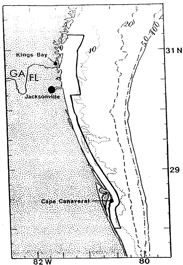
Figure 8. The area designated as critical habitat in the Southeastern United States includes waters between 31^{\circ}15'N (approximately located at the mouth of the Altamaha River, GA) and 30^{\circ}15'N (approximately Jacksonville, FL) from the shoreline out to 15 nautical miles offshore, and the waters between 30^{\circ}15'N and 28^{\circ}00'N (approximately Sebastian Inlet, FL) from the shoreline out to 5 nautical miles.
